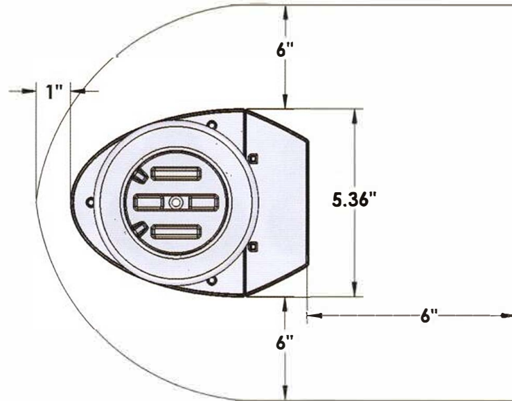
SPACE REQUIRED FOR UNIT MOUNTING
