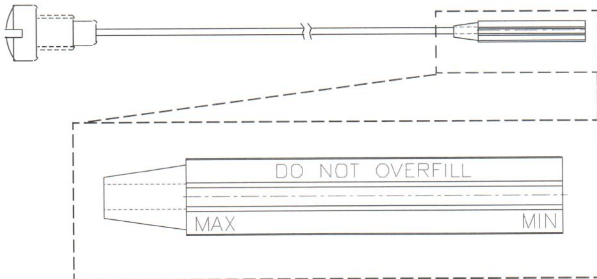
FIGURE H1 DIPSTICK DETAILS
